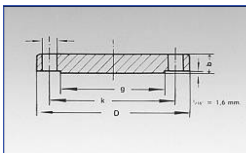
Flange Blind - Flange Cieche ASA 150 lb. ASA B 16.5 - ASTM 105 - Gr. 1
